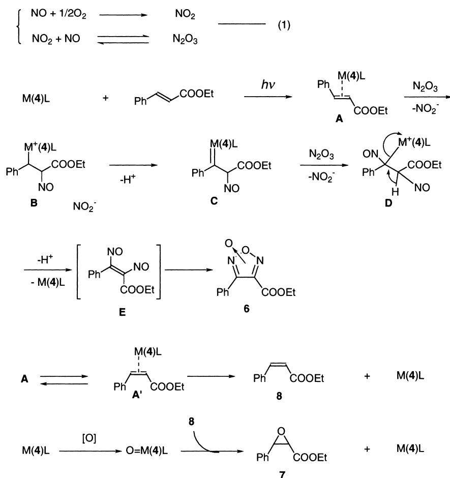
Scheme 2. A possible reaction mechanism for the formation of furoxan 6–8.
