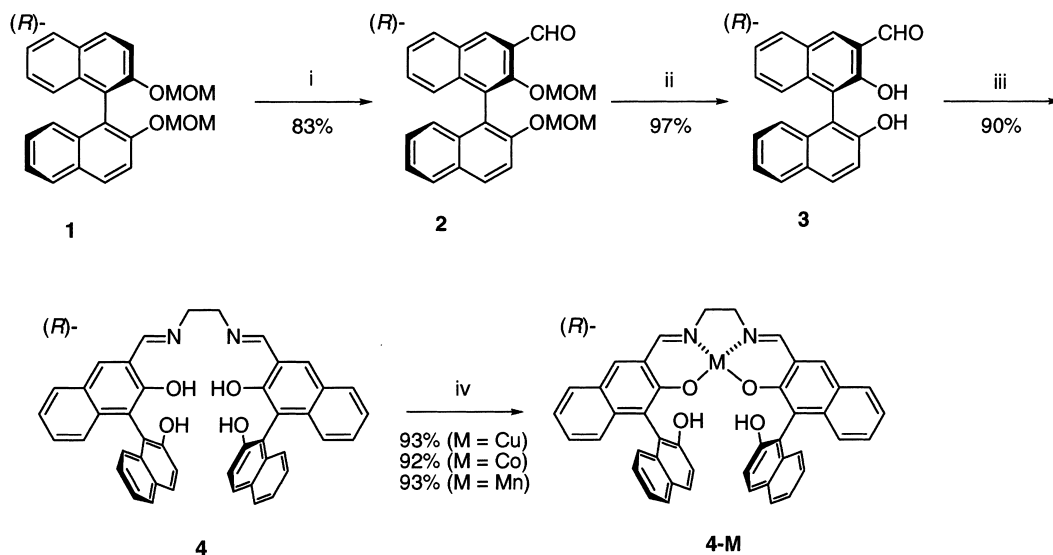
Scheme 1. Synthesis of metallosalen complexes 4-M : (i) n -BuLi, DMF/THF, (ii) HCl, i -PrOH/CH 2 Cl 2 , (iii) ethylenediamine/benzene, (iv) M(OAc) 2 /CH 2 Cl 2 .
