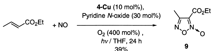
Scheme 3. Reaction of ethyl crotonate with nitrogen monoxide.
